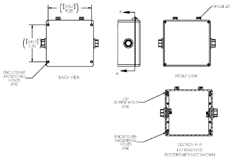
Polyester NEMA 4X, IP66, for Hazardous Locations
